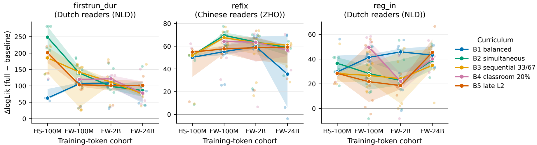
d1: \Delta\log\text{Lik} per eye-tracking measure (one reader L1 per measure, chosen by data availability) (trend lines drawn only where n \geq 3 models per cell)
